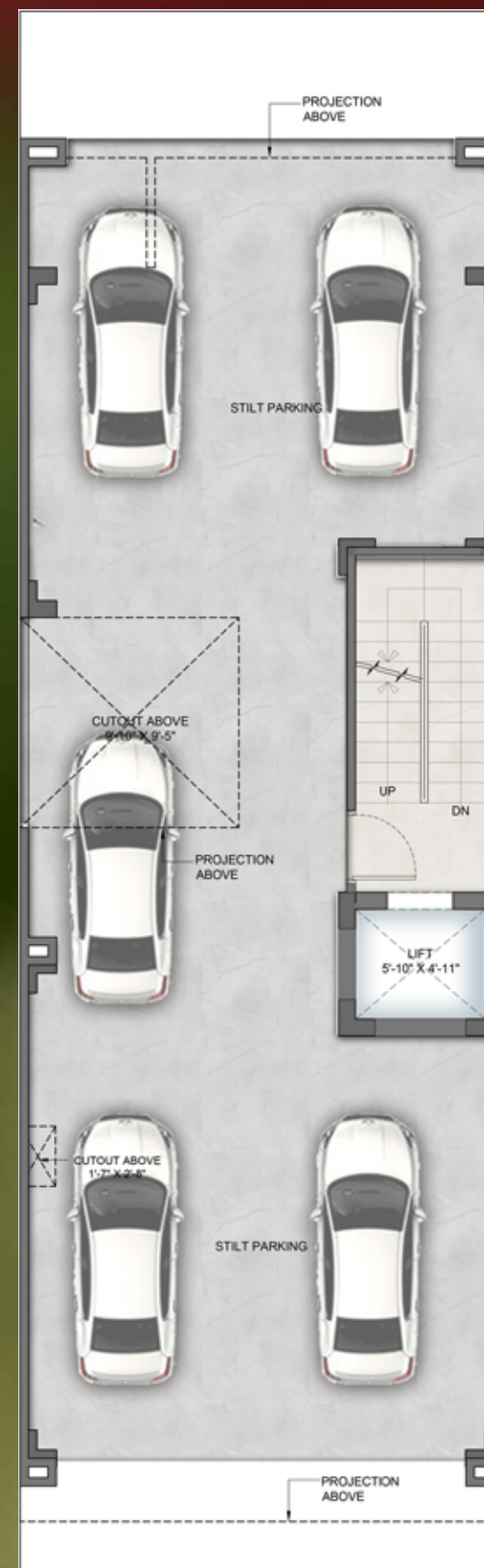
Stilt Floor Plan
